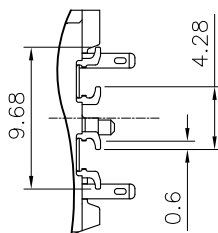
SMT TAIL DIMENSION
